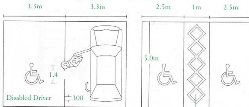
Marked out shared space between 2 standard bays
