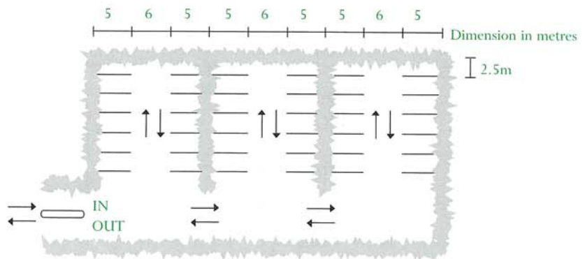
Cul-de-sac aisle system
