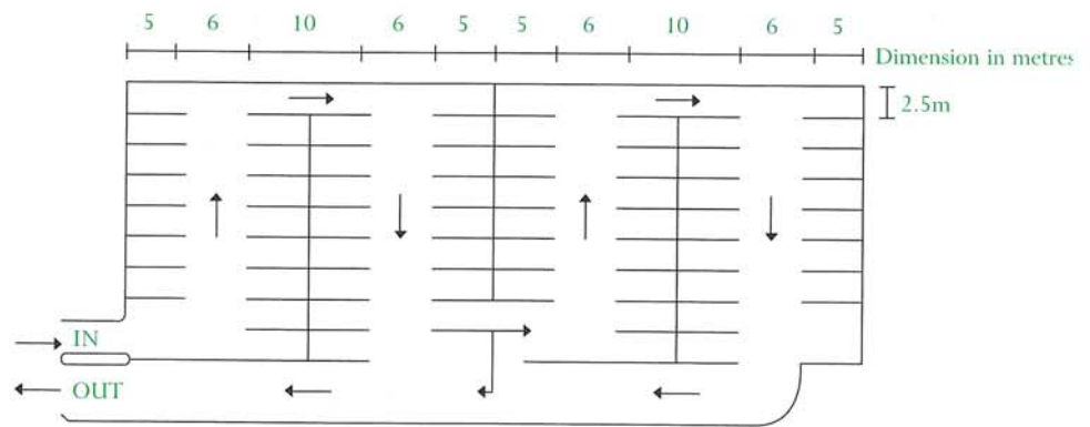
Single aisle one-way system
